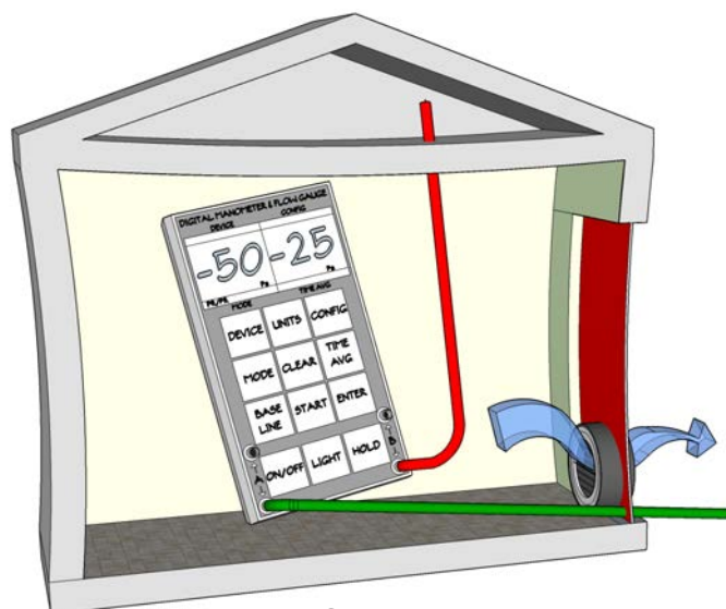
FIG. 5-3. House Pressure WRT Outside (Channel A) and WRT Attic (Channel B)
