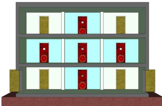
Figure 16-21. Multifamily Adjacent Spaces Guarded Test
