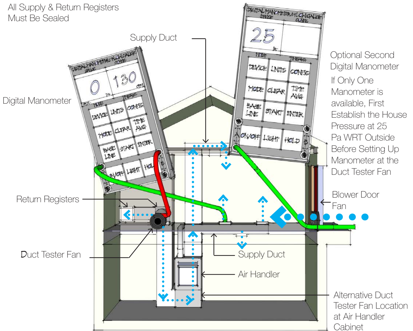
FIG. 7-12. Leakage to Outside Test
