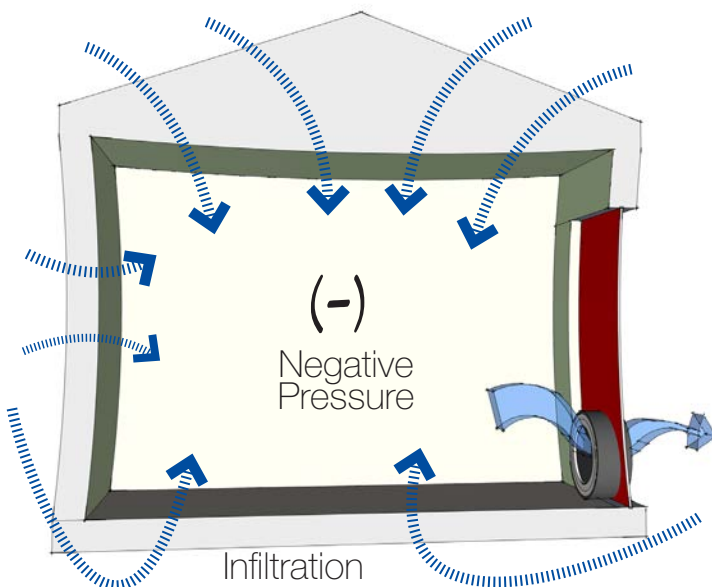
Figure 6-7. Depressurization Test
