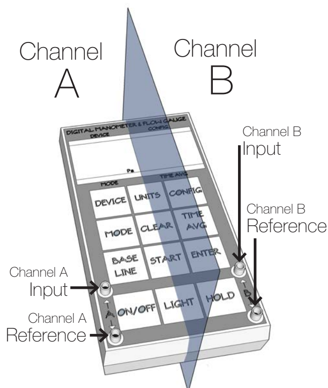
FIG. 5-2. Two-Channel Digital Manometer
