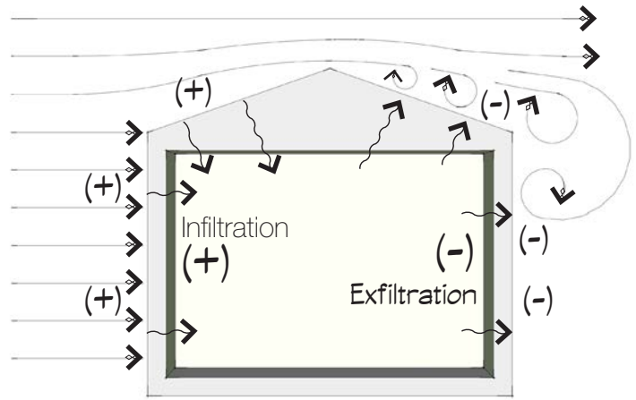
Figure 4-5. Wind Effect
