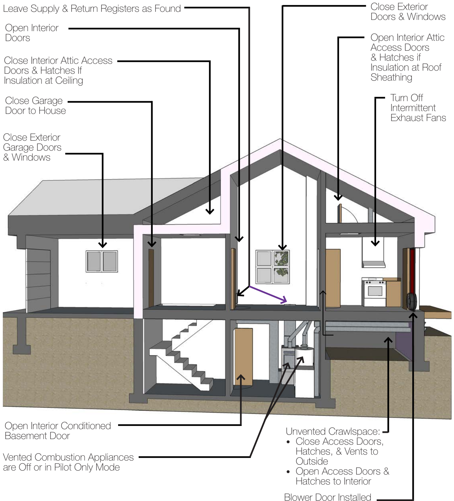
Figure 6-10. Blower Door Test Building Preparation Common Configuration
