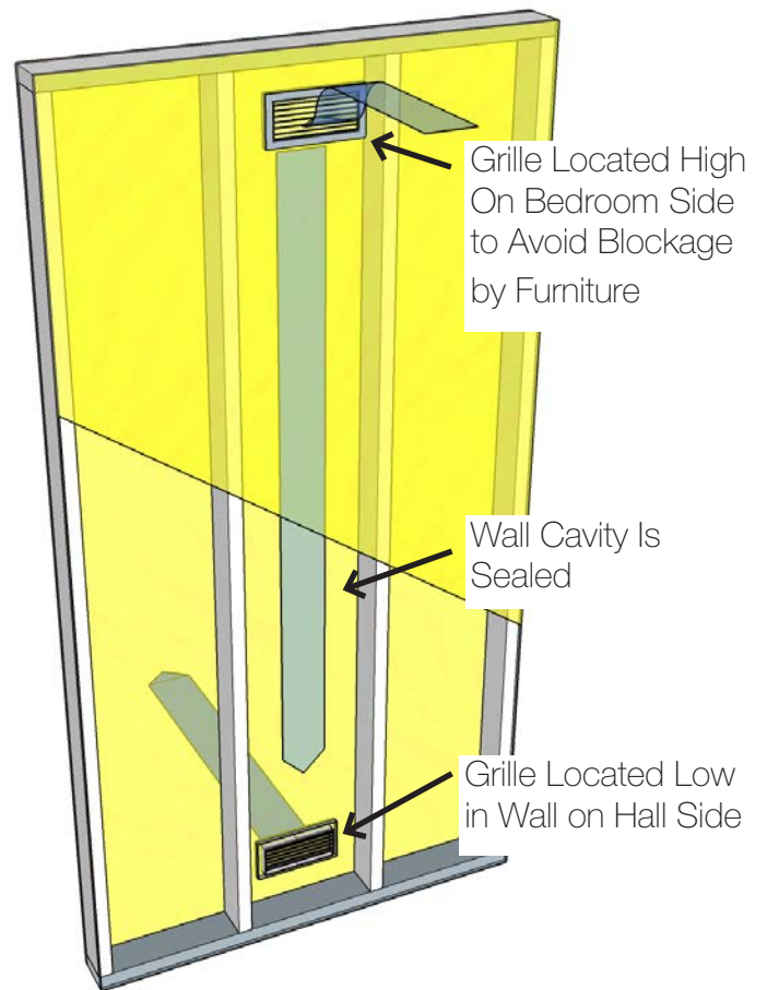
Transfer Grill
