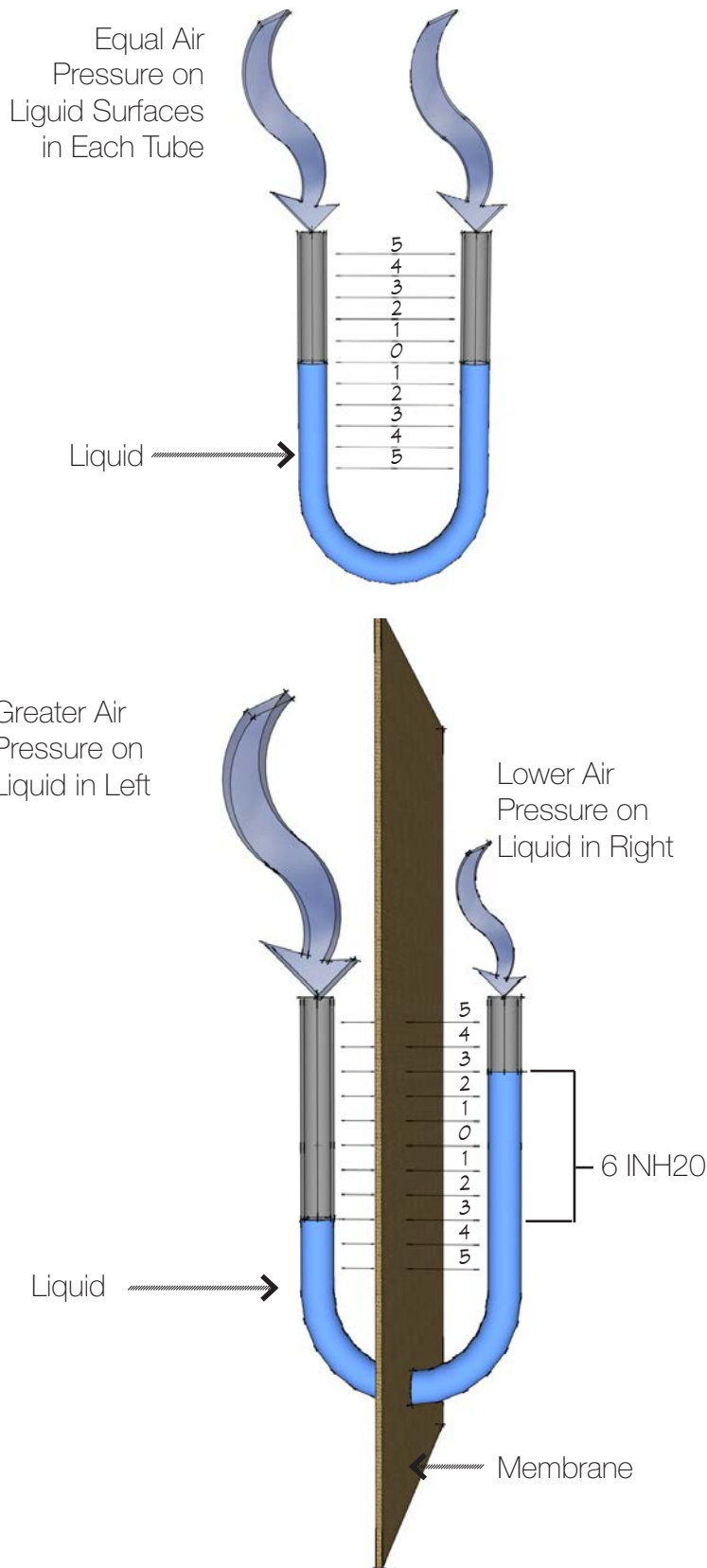
Figure 4-1. Conceptual Manometer
