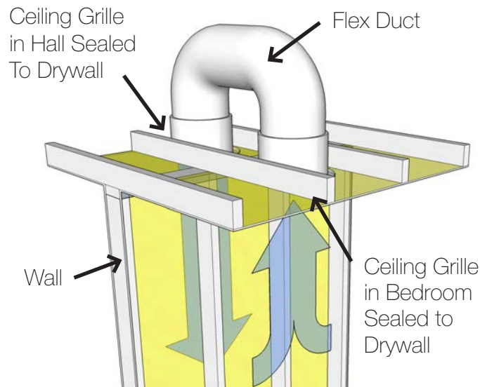
Crossover Duct
